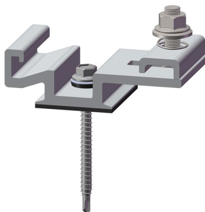
ezClick connection for T-Rail, V1.1 Part No.: ER-EZC/T/V1R1 (Barcode:10-007-01100)
