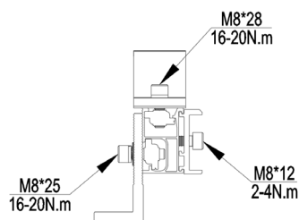
ER-I-05 and ER-I-25 (with ECO rail splice, ER-SP-ECO)
