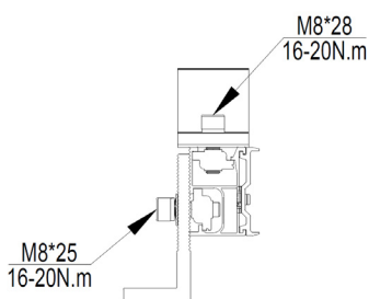
ER-I-05 and ER-I-25 (with Elite rail splice, ER-SP-ELT)
