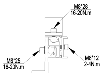
ER-I-05/CM (with ECO rail splice, ER-SP-ECO)
