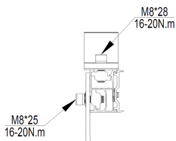
ER-I-01 and other tile interfaces (with Elite rail splice, ER-SP-ELT)
