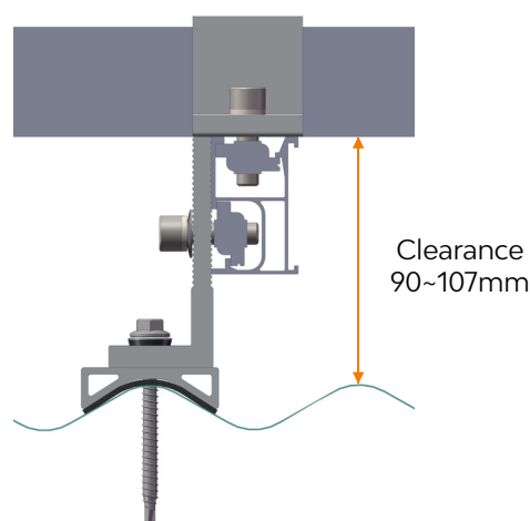
The rail is parallel to the Rib of metal sheet roof
