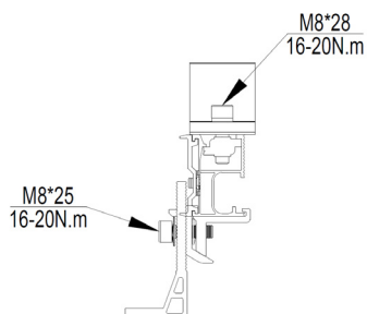
ER-I-05A/EZC/ECO (with Elite rail splice, ER-SP-ELT)
