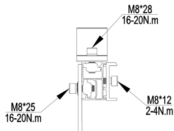
ER-I-01 and other tile interfaces (with ECO rail splice, ER-SP-ECO)
