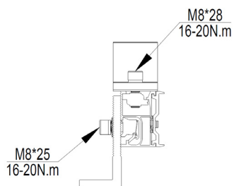
ER-I-05/CM (with Elite rail splice, ER-SP-ELT)
