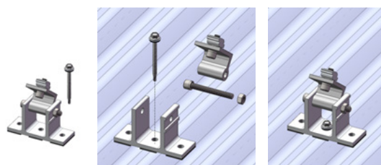
Figure 5.7b (Front Leg Installation with Single Screw)
