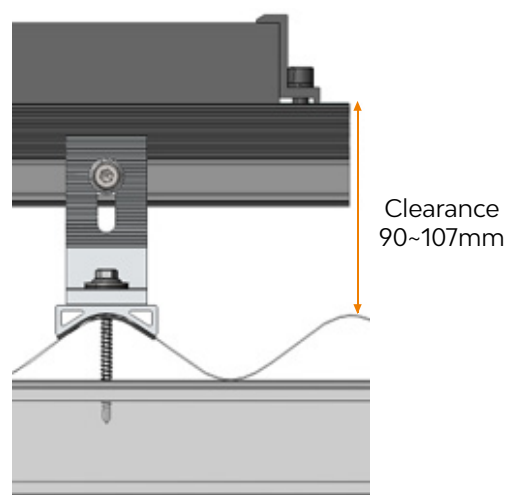
The rail is perpendicular to the Rib of metal sheet roof
