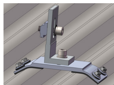
Rail running parallel to roof rib
