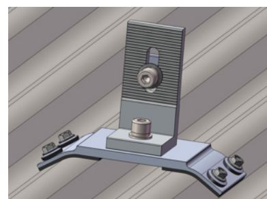
Rail running perpendicular to roof rib
