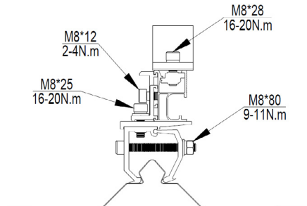
ER-I-34 with Cross Connector Clamp (with ECO rail splice, ER-SP-ECO)
