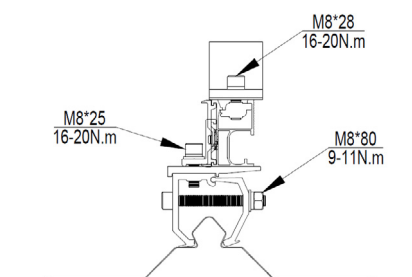
ER-I-34 with Cross Connector Clamp (with Elite rail splice, ER-SP-ELT)
