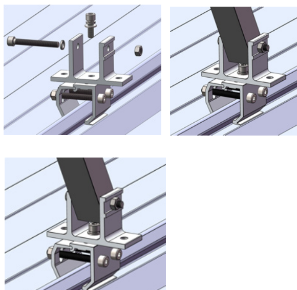
Figure 5.3f Non-preassembly Rear Leg Installation with Brooklyn Klip-lok Interface
