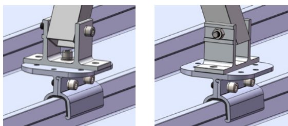
Figure 5.3h Rear Leg Installation with Other Klip-lok Interface
