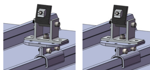
Figure 5.3b Front Leg Installation with Other Klip-lok Interface
