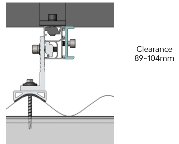
The rail is parallel to the Rib of metal sheet roof
