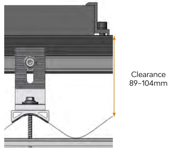
The rail is perpendicular to the Rib of metal sheet roof
