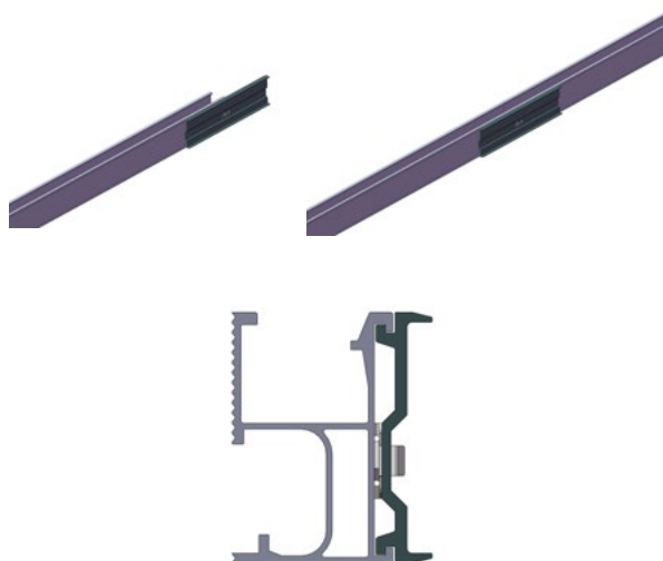
Elite-rail installation with Elite rail splice
