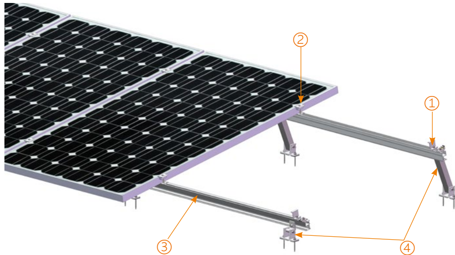
1. End Clamp 2. Inter Clamp 3. Elite Rail 4. Fixed Tilt Legs
