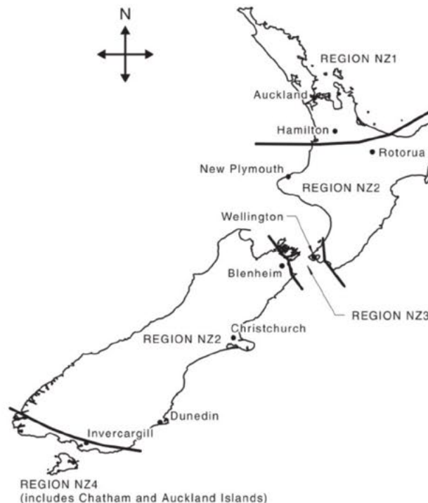
Figure 3.1(B) — Wind regions — New Zealand
