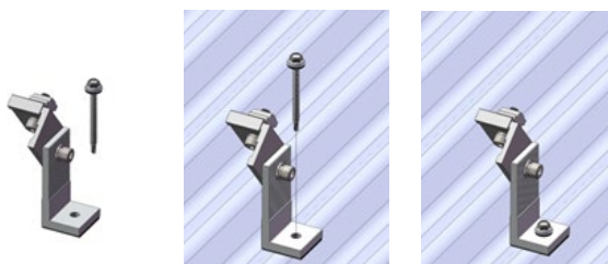
Figure 3 (Tin Foot Front Leg Installation)
