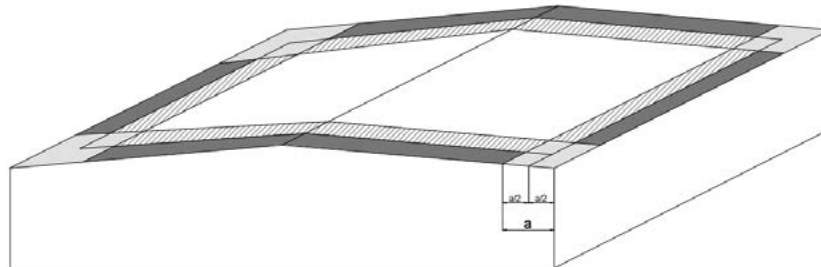
Roof Pitch <math>< 10^\circ</math>
