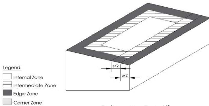
Flat/Mono – Slope Roof \geq 10^\circ
