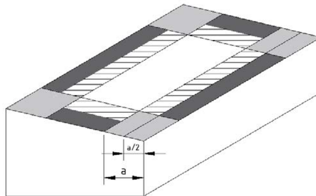
Flat/Mono – Slope Roof <math>< 10^\circ</math>
