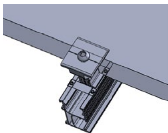
End Clamp
