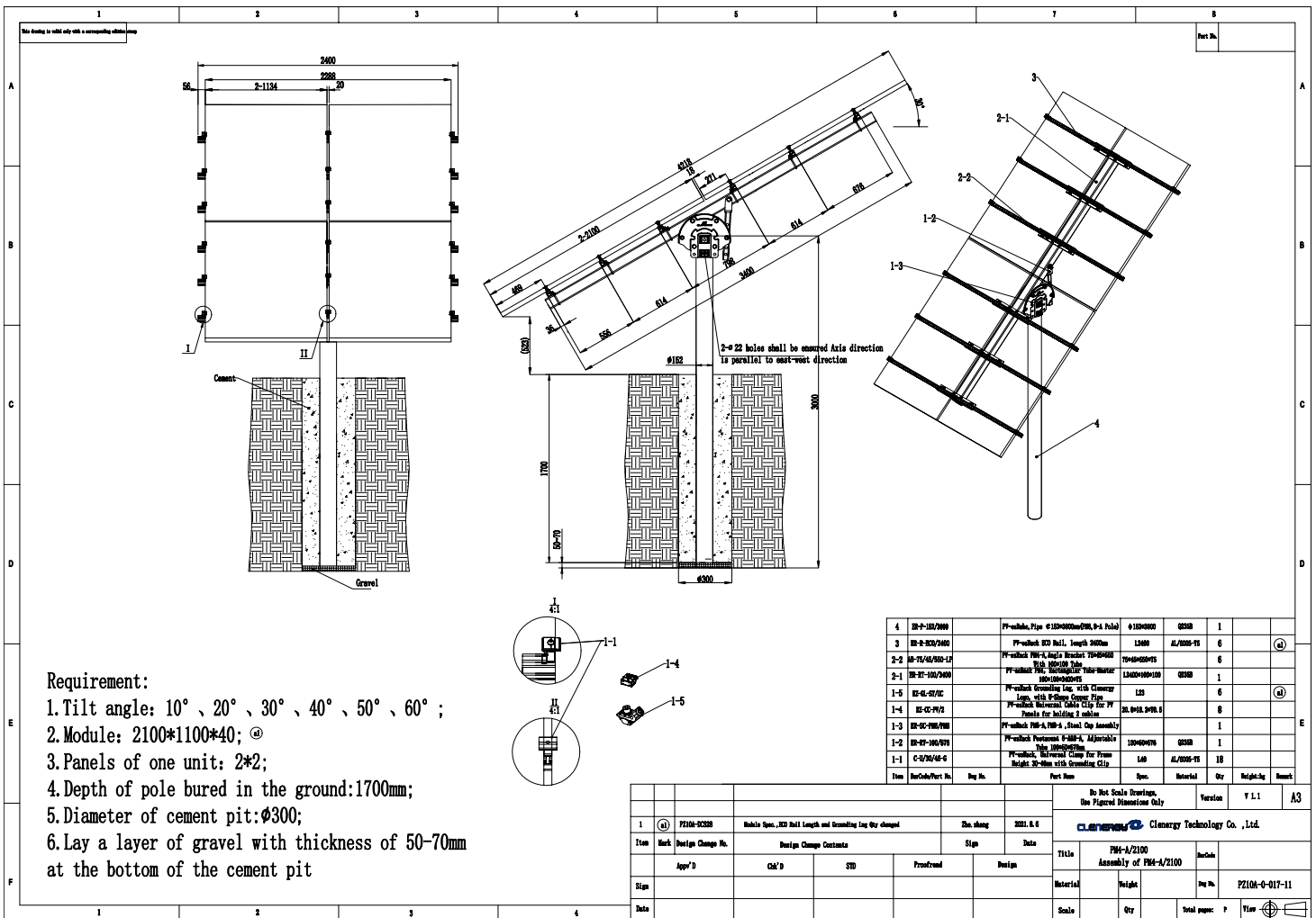
Figure A1 – Clenergy Post Mount PM4-A/XL System Design Drawing (30 Degree Tilt Case)
