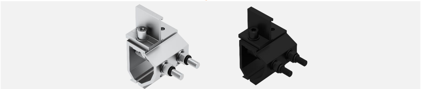
Universal Klip-lok Interface pre-assembly with Cross Connector Clamp
