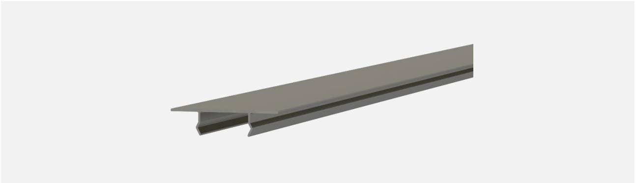
Cover for MT-Rail Cable Tray, length 855mm Part No.: CO-MT/855
